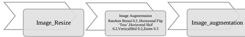
Gambar 2. Tahapan Image Augmentation
